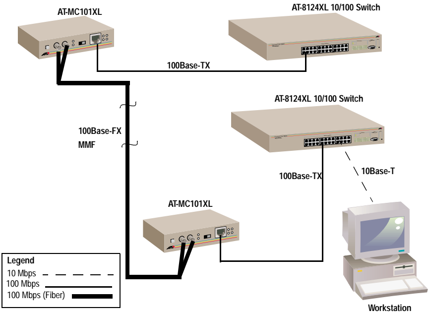
Figure 10 AT-MC101XL Back-to-Back Configuration
