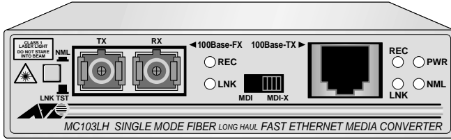
Figure 4 AT-MC103LH (SC single mode connector)
