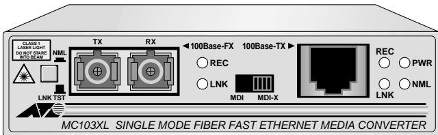
Figure 3 AT-MC103XL Front Panel (SC single mode connector)
