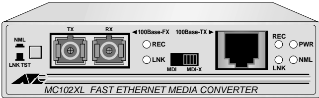
Figure 2 AT-MC102XL Front Panel (SC multimode connector)
