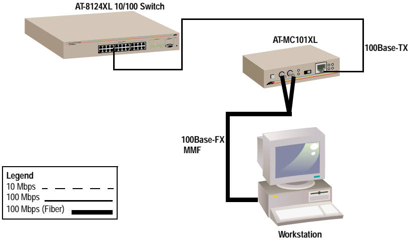
Figure 9 Connection to Workstation and Switch
