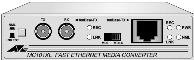
Figure 1 AT-MC101XL Front Panel (ST multimode connector)
