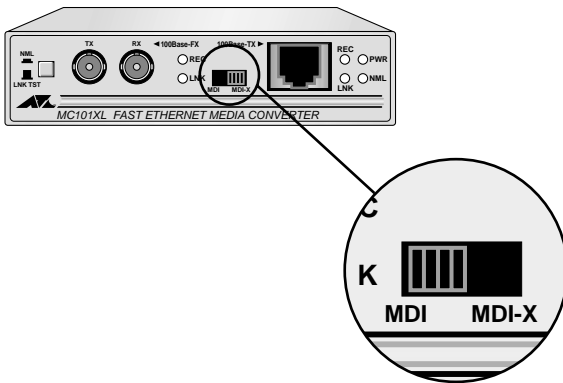
Figure 7 MDI/MDI-X Switch
